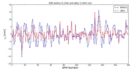
Figure 7: Preliminary test of slow orbit feedback.
