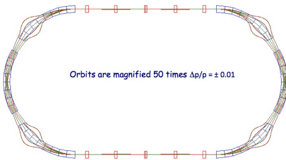
Figure 4: Closed orbit dependence on momentum.
