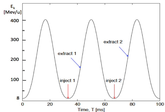
Figure 1: Three cycles of the iRCMS show the energy flexibility. Beam is injected on cycles 1 and 2 (“inject 1” and “inject 2”). The relative timing of the extraction is trivially changed from cycle to cycle, to adjust the extraction energy (“extract 1” and “extract 2”).
