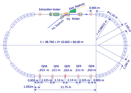
Figure 2: A layout of the synchrotron.
