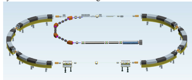
Figure 5. Detail layout of the synchrotron.
