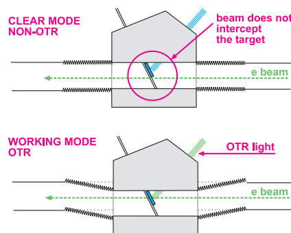
Figure 1: The OTR body is lowered to enable the target to intercept the beam.
