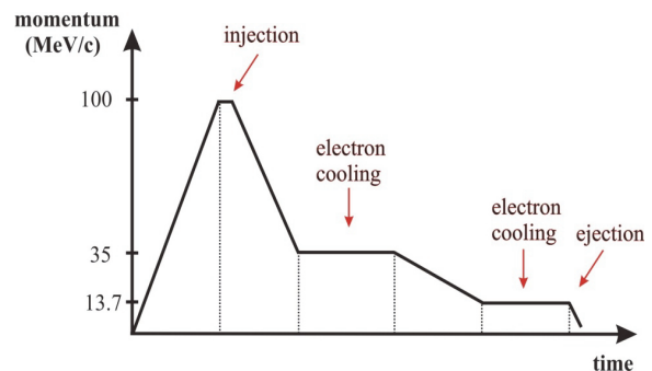
Figure 2: ELENA cycle.
