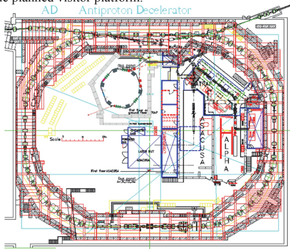
Figure 1: ELENA and AD layout.
