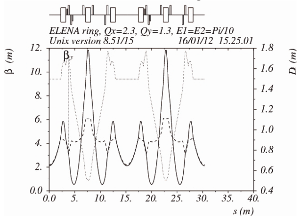
Figure 3: ELENA ring lattice functions.
