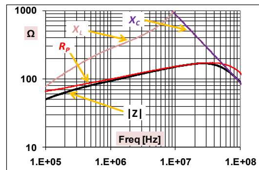
Figure 1: Finemet ® loaded resonator typical response.
