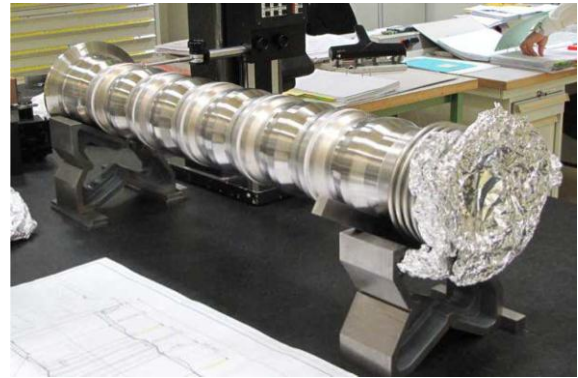
Figure 11: 5 gaps vacuum chamber.
