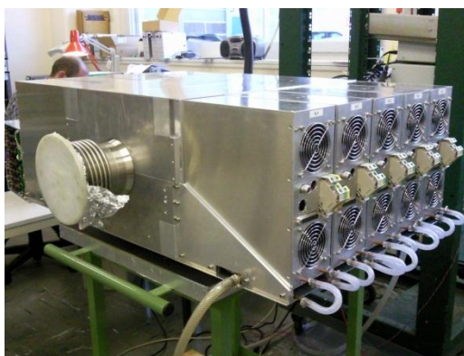
Figure 10: Fully assembled system including the power stages.
