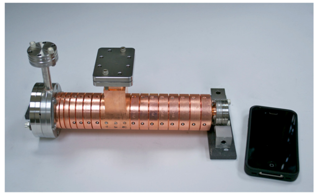
Figure 4: Completed, brazed first section of the 1 MeV MicroLinac, with mobile phone shown for scale.
