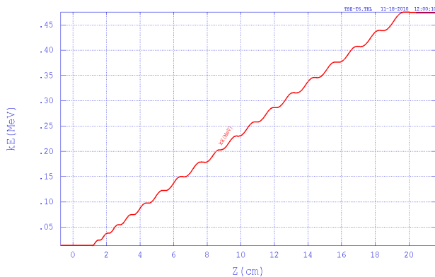
Figure 3: PARMELA simulation of the first section of the 1 MeV MicroLinac, showing 500 keV energy gain.
