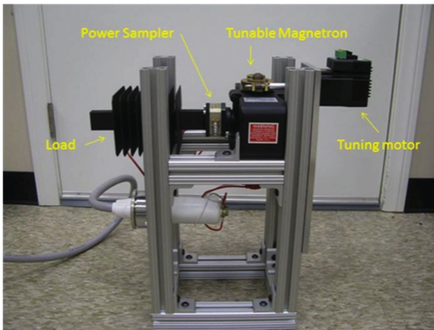
Figure 2: Tunable X-band magnetron being used for initial prototype testing.
