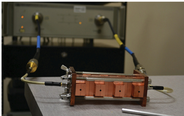
Figure 7: Cells of the 2 MeV MicroLinac undergoing initial cold-testing.
