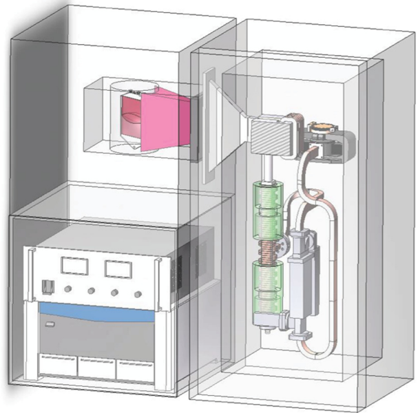
Figure 8: Conceptual design of the 2 MeV MicroLinac configured in a self-contained irradiator.
