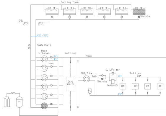
Figure 9: Cooling-water system.
