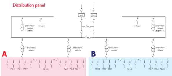
Figure 7: Main substation single-line diagram.
