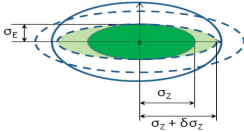
Figure 1: Distortion of the RF bucket and the bunch longitudinal phase space due to RF voltage modulation are schematically shown.
