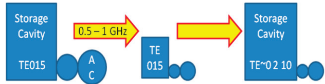
Figure 2: Two step processes of cavity scaling and modification for R/Q reduction is schematically shown.
