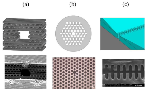
Figure 1: Three dielectric laser accelerator topologies: (a) a 3D silicon photonic crystal structure, (b) a hollow-core photonic bandgap fiber, and (c) a dual-grating structure, showing conceptual illustration (top) and recently fabricated structures (bottom).
