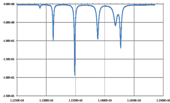
Figure 2: Complete RF spectrum.
