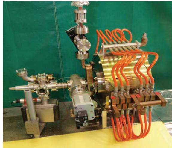
Figure 1: RF gun test assembly.
