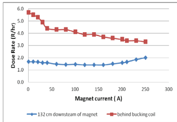
Figure 8: Radiation dose rate vs. solenoid field.
