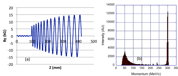
Figure 4: (a) Optimized planar undulator field design and (b) resulting IFEL momentum spectrum using the existing LLNL laser parameters.
