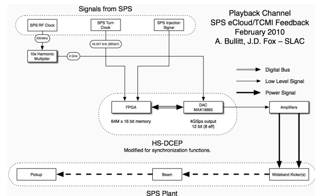
Figure 1: Block diagram of the excitation system developed for use at the SPS. The timing functions are synchronized with the machine RF, so that the excitation can be specific for a selected bunch, and the digital memory stores up to 15,000 turns of user-defined excitation signals.
