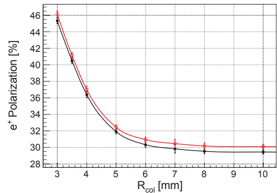
Figure 9: Positron polarization vs aperture radius of photon collimator.
