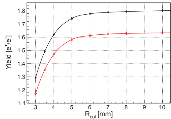
Figure 8: Yield vs aperture radius of photon collimator.
