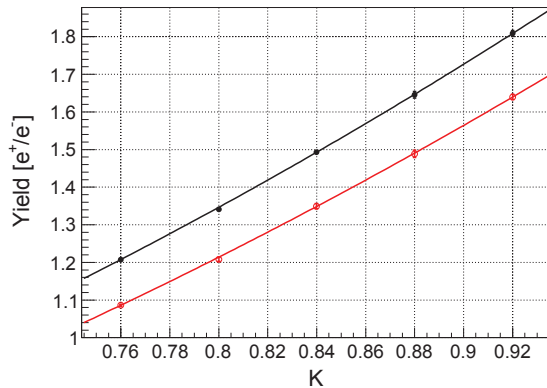
Figure 6: Yield vs undulator K value.
