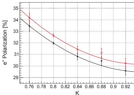
Figure 7: Positron polarization vs undulator K value.
