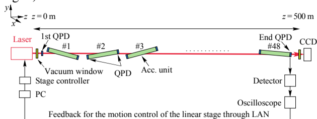
Figure 4: Feedback control system for stabilizing the laser pointing at the end QPD.
