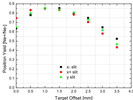
Figure 4: Positron yield (number of positrons per electron) as a function of target offset. The FC center is 2 mm away from the center axis. The black, red and green marks represent the slit orientation of x-, x+ and y respectively, as marked in Fig. 2
