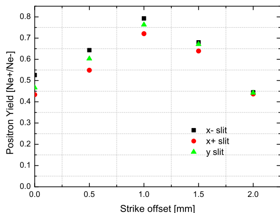
Figure 5: Positron yield as a function of electron bombardment position respect to the target center. Strike offset equals 0 is the target center and the primary electron beam's moving direction is toward to the central axis. The black, red and green marks represent the slit orientation of x-, x+ and y respectively, as marked in Fig. 2
