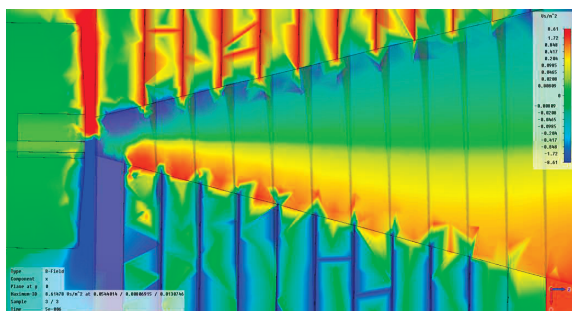
Figure 3: CST 2D FC transverse field distribution.
