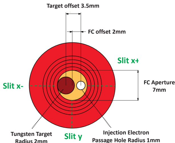
Figure 2: SuperKEKB positron target geometry. The red part represent the FC, yellow is the cooling copper and brown is the tungsten target. The injection electron passage hole is shown in white. The green dash lines are the three possible slit orientation directions.
