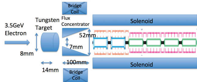
Figure 1: Schematic view of SuperKEKB positron source configuration [5].
