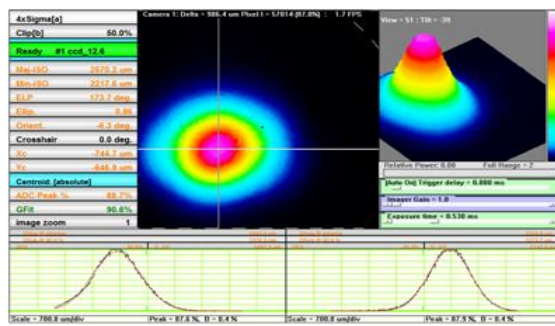
Figure 2: Measured laser beam transverse profile.
