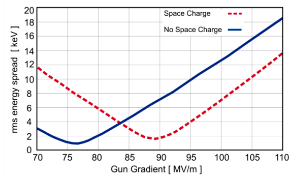
Figure 3: The beam RMS energy spread at the gun exit versus acceleration gradient. The results with (red) and without (blue) space charge effects are shown.
