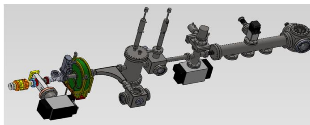
Figure 1: The schematic layout of AREAL machine.
