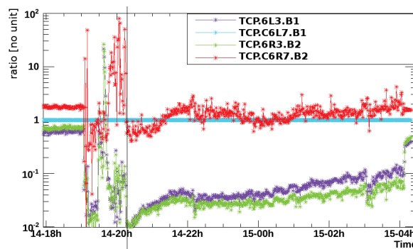
Figure 6: BLM signal at the TCPs normalised to the signal at TCP.C6L7.B1 versus time, during fill #2628, 2012/05/16. The sharing between B1 and B2 in IR7 changes with time. The contribution of IR3 keeps increasing during the fill.
