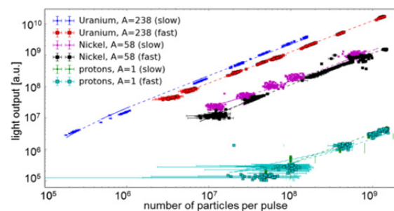
Figure 3: Light output from a P43 phosphor screen for fast and slow extraction irradiation by protons (fast 299.8 MeV, slow 299.4 MeV), Nickel (fast 297 MeV/u, slow 290 MeV/u) and Uranium (fast 340 MeV/u, slow 320 MeV/u). The vertical error bars for fast extraction of protons are related to the current transformer detection threshold of 1.5 \times 10^7 ppp.
