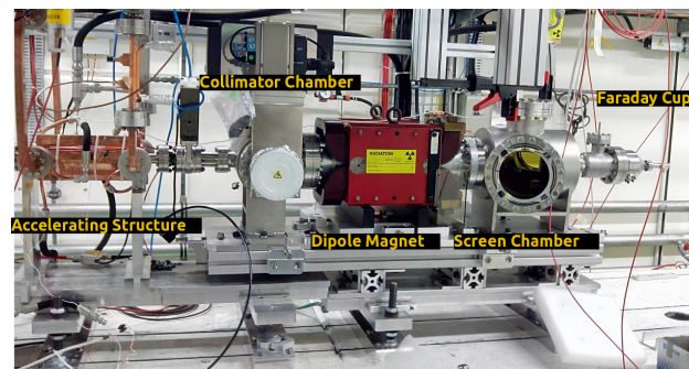
Figure 3: The new diagnostic setup during installation. From the left is shown the accelerating cavity followed by the first vacuum chamber housing the collimator, then dipole magnet and chamber with the fluorescent YAG screen with the view-port for the camera (the camera with the optical line is not in the picture). There is a special Faraday cup at the right side, that closes the setup.
