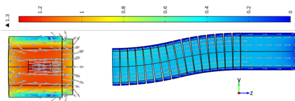
Figure 10: The Chicane magnets form a bent solenoid.
