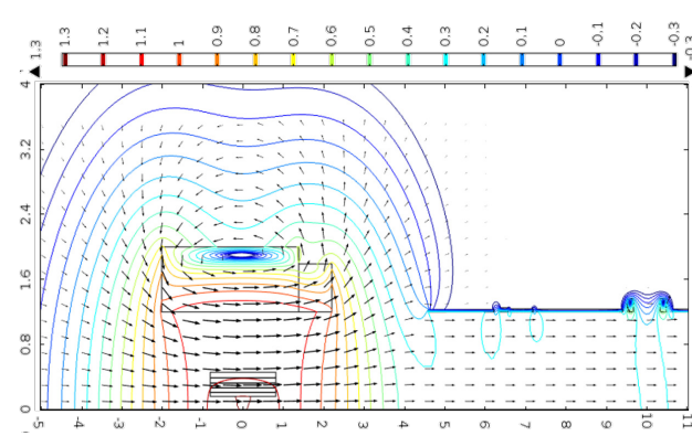
Figure 6: Field map of the taper region for 0 < r < 4 m and -5 < z < 11 m.
