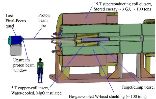
Figure 2: Sketch of the Target System concept.
