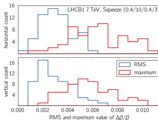
Figure 2: Distribution of the rms and maximum beta-beating for the squeezed optics.
