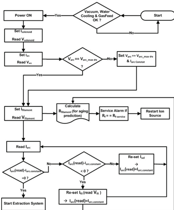
Figure 7: Plasma generator proposed control loop.
