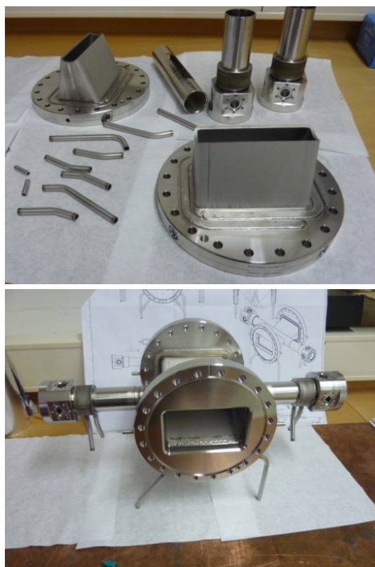
Figure 2: Fabrication of plasma cell body. a) fabricated parts. b) finished cell body, welded together.
