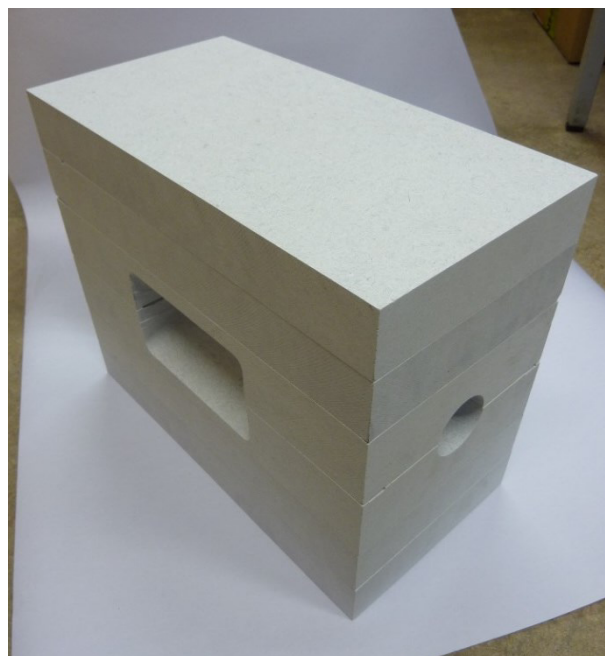
Figure 4: Heat insulation for the plasma cell.
