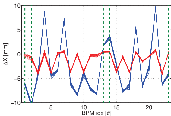
Figure 5: Difference between the first and second turn horizontal orbit of a short (< 280 ns) pulse circulating in the CR. Each line is an average over 10 consecutive pulses. The blue and red lines are respectively before and after orbit closure correction.
