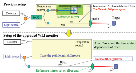
Figure 1: Setup of the previous WLI monitor (above) and upgraded WLI monitor (below).
