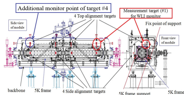
Figure 4: Detailed cross sections of the cERL main linac cryomodule with 8 alignment targets including the monitoring target (#1) & (#4) by upgraded WLI monitor.
