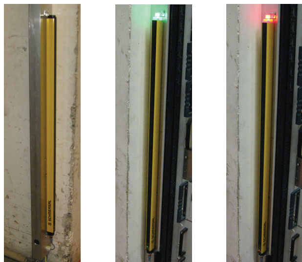
(a) The emitter of the light grid system. (b) The acceptor of the light grid has a green light to show that nobody was detected by the system. (c) The red light of the acceptor shows that someone has interrupted the signal.
