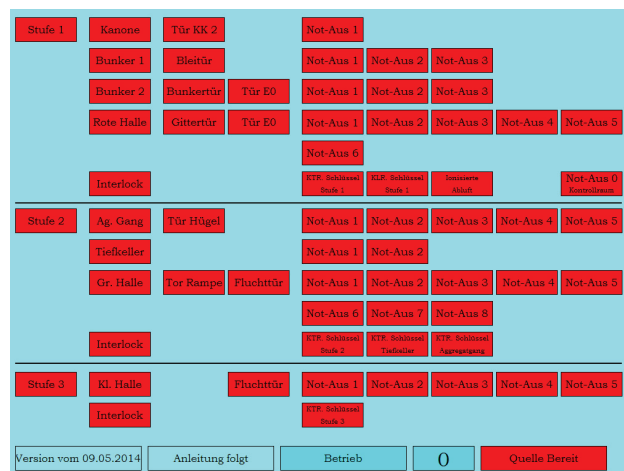
Figure 5: This screen shows the three levels of the personnel interlock subsystem with their conditions, mainly the status of emergency shutdown buttons and doors.
