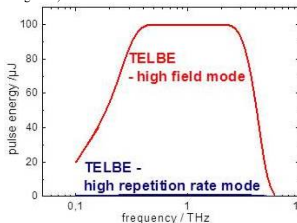
Figure 1: Design parameters for the super-radiant THz sources at ELBE postulated from electron beam dynamic simulations [7]. The high field mode utilizes the new SRF gun [8] and can operate up to a repetition rate of 500 kHz. The high repetition rate mode utilizes the standard thermionic injector and allows operation up to repetition rates of 13 MHz.
