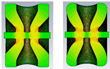
Figure 6: Design change of SSR1: flat end-walls (left) and round end-walls (right).
