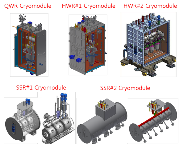
Figure 7: RISP Cryomodules.
