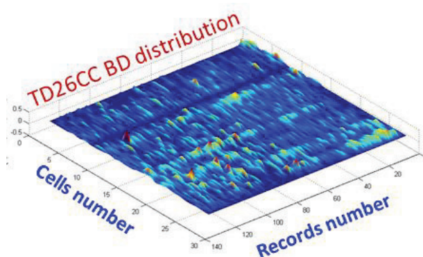
Figure 4: Breakdown distribution as a function of cell number and of time, in 8 hour records.
