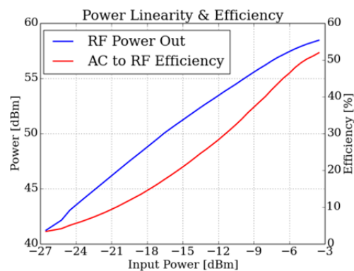
Figure 5: Output power and efficiency vs. input RF power.
