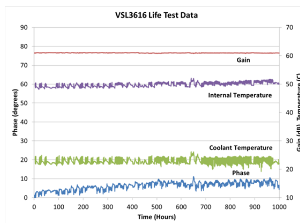
Figure 10: Phase, gain and temperature over 1000 hours.
