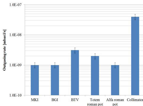
Figure 5: Outgassing rates after bake out of some LHC machine devices tested during LS1 (MKI: injection kicker; BGI and BTV: beam monitors; Totem and Alpha roman pot: detectors).
