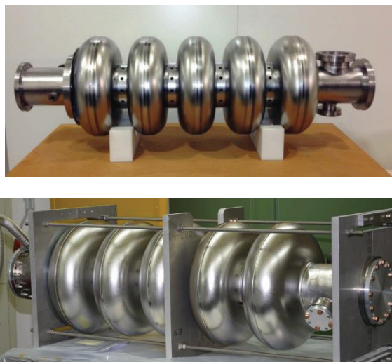
Figure 1: ESS high beta prototype cavity n°1 (up) and n°2 (down) at factory before shipment.
