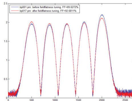
Figure 2: On-axis E-field profile of cavity n°1 before (blue) and after (red) tuning (arbitrary units in both axis).
