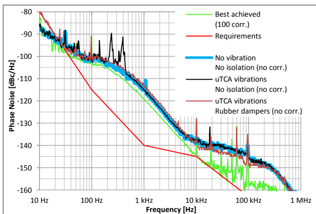
Figure 5: Phase noise under vibrations.
