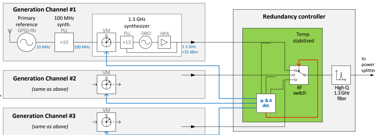
Figure 3: Block diagram of MO. Redundancy idea highlighted - drift compensation, phase and amplitude fail detection, fast RF switch and 1.3 GHz filter with high-Q resonator.
