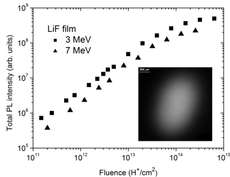
Figure 4: Integrated visible photoluminescence signal as a function of the 3 and 7 MeV proton fluence in irradiated 1 \mu\text{m} thick LiF films grown on a glass substrate.
