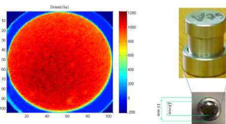
Figure 3: left) Spatial dose distribution on Gaf-Chromic EBT3 film: the irradiated area has a uniformity of 90%; right) Sample holder for cells.
