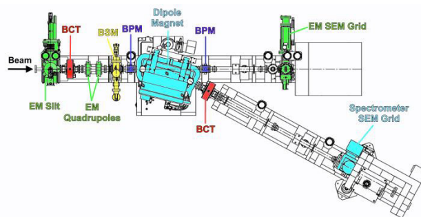
Figure 2: Movable diagnostic bench for 3MeV and 12MeV beam measurements.
