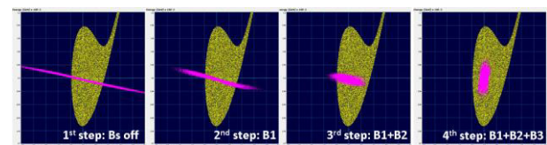
Figure 4: Comparison of the beam longitudinal phase space (in purple) with the tank1 longitudinal acceptance plot (in yellow). From left to right: all bunchers off, first buncher on, first two bunchers on, all bunchers on. For each plot, the axes are \Delta\phi and \Delta E with the range of \pm 200^\circ and \pm 0.3\text{MeV} respectively.
