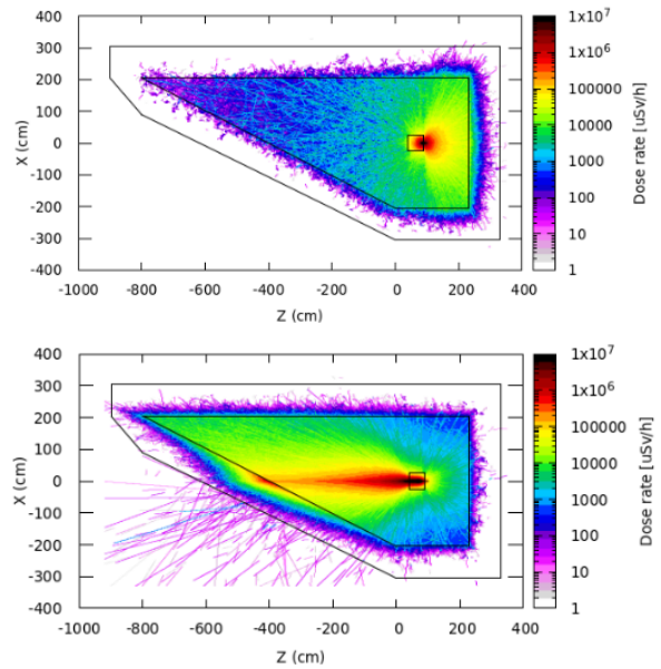
Figure 4: Total effective dose equivalent maps from different target, lead(top) and graphite (bottom).
