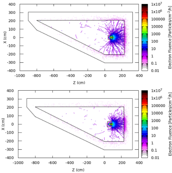
Figure 6: Electron fluence from combined structures.
