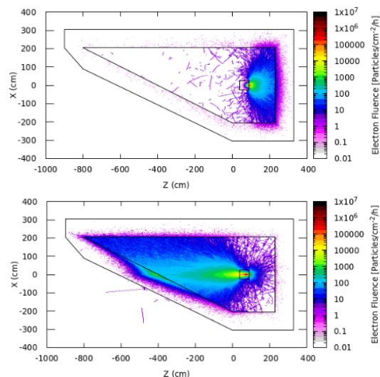
Figure 1: Electron fluence from different target, lead(top) and graphite (bottom).
