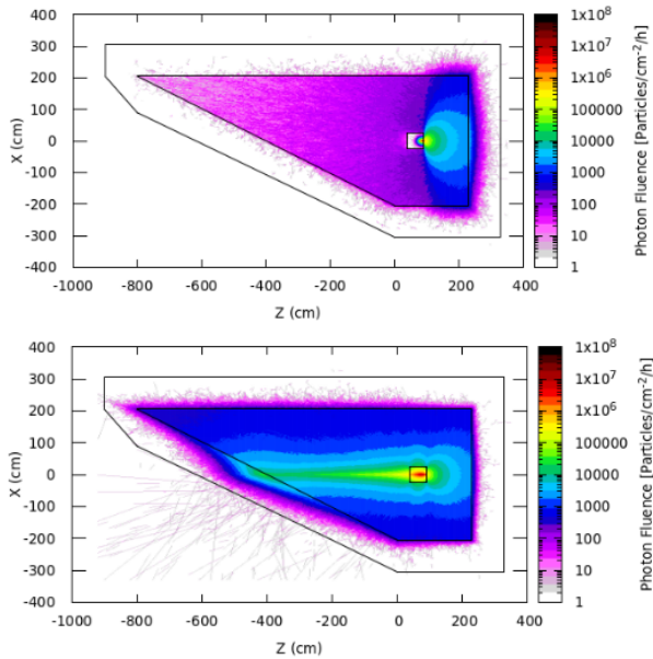
Figure 2: Photon fluence from different target, lead(top) and graphite (bottom).
