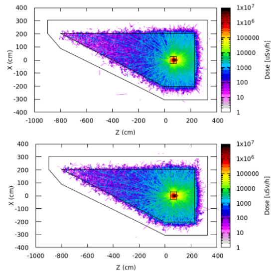
Figure 9: Total effective dose equivalent maps from combined structures.
