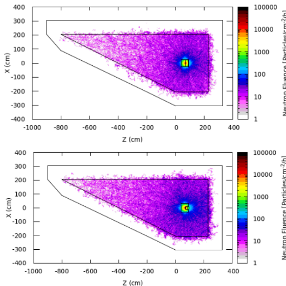
Figure 8: Neutron fluence from combined structures.
