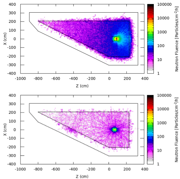
Figure 3: Neutron fluence from different target, lead(top) and graphite (bottom).
