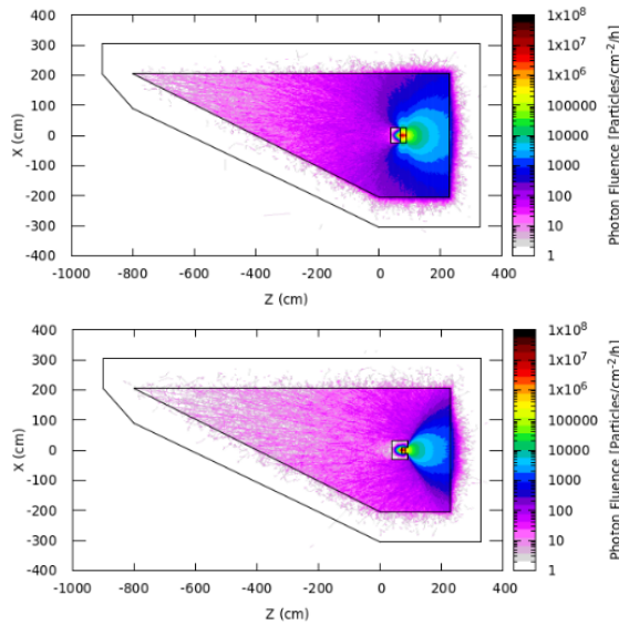
Figure 7: Photon fluence from combined structures.
