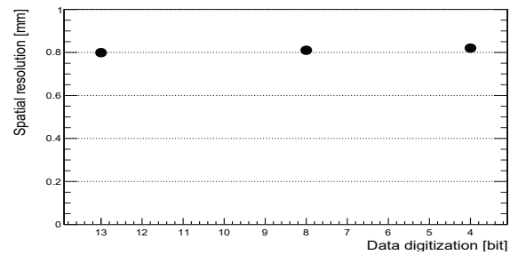
Figure 7: Measured spatial resolution with different data digitization.
