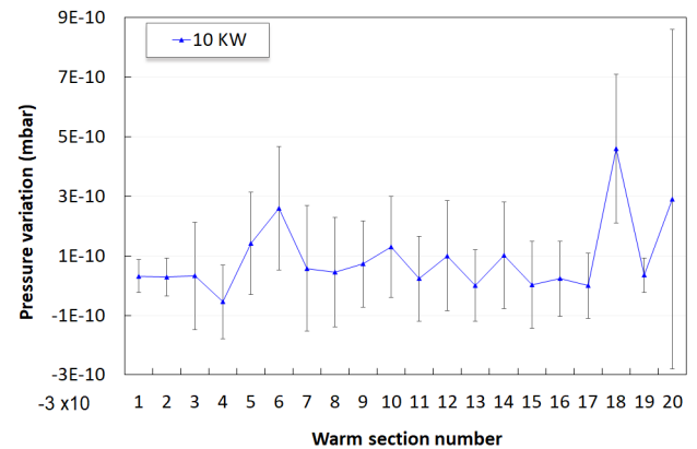
Figure 7: Pressure variation at 10 kW beam power.
