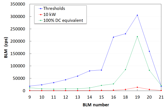
Figure 6: BLM count rate: thresholds (blue), 10 kW deuteron beam (red) and extrapolation to 200 kW (green).
