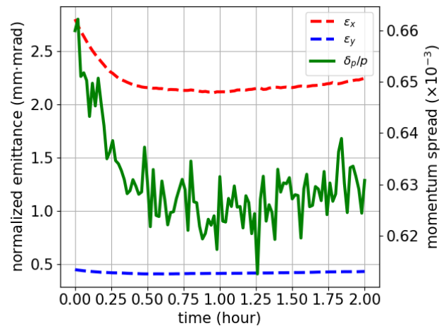
Figure 3: The evolution of the horizontal ( \epsilon_x ), vertical ( \epsilon_y ), and longitudinal ( \delta_p/p ) proton beam emittance during cooling. Upper plot: D_t = 0 m; bottom plot: D_x = 2.5 m, D_y = 0.5 m and IBS coupling factor = 0.2.
