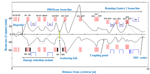
Figure 3: The new beam optics including a scattering foil transports 67 \pi \text{ mm} \cdot \text{mrad} in X-plane and 139 \pi \text{ mm} \cdot \text{mrad} in Y-plane up to scattering foil location and transports almost 140 \pi \text{ mm} \cdot \text{mrad} (in both planes) from scattering foil to isocenter. The beam envelopes show the beam size in 2-sigma values and the dispersion (dashed line) along PSI's ESS beam line (The lower half of figure shows beam envelope in X-plane (bending plane) and the upper half shows envelope in Y-plane).
