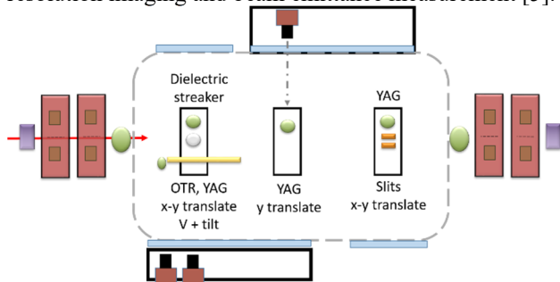
Figure 4: Proposed experimental diagnostic layout in FEC2.
