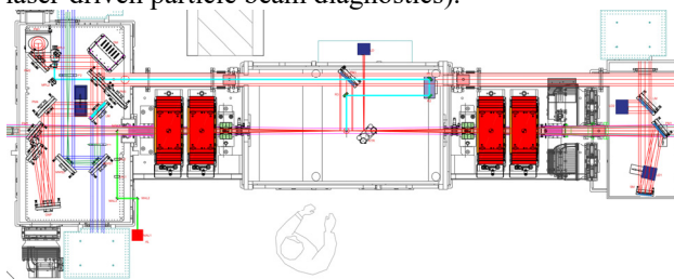
Figure 2: Laser transport schematic in the FEBE hutch.
