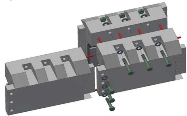
Figure 6: Modular permanent magnet spectrometer design with precision metal dowels.
