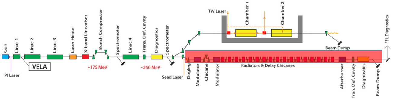
Figure 1: Overview of the CLARA and FEBE beamlines. The proposed CLARA FEL location is highlighted in red.
