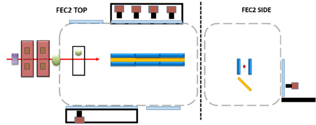
Figure 5: Spectrometer with screen and cameras for wide-energy spectrometry in FEC2.
