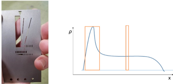
Figure 3: Mask design (left) and desired energy spectrum of the electron bunch at the position of the mask to generate drive-/main-bunch pairs (right).
