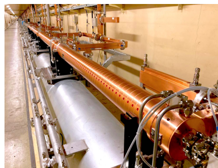
Figure 4: New S-band accelerating structures installed in the tunnel.
