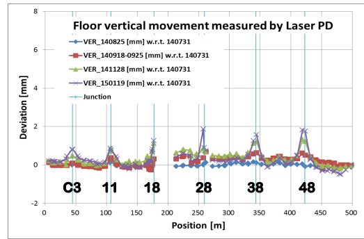
Figure 3: Seasonal floor movement in LINAC tunnel.
