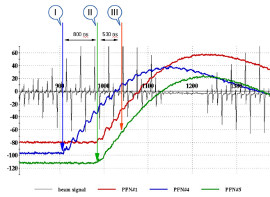
Figure 2: Timeline of a typical Abort Kicker pre-fire. Module 4, in blue, fired by itself (I) and 800 ns later the other modules re-triggered (II), here, only modules 1 and 5 are shown in red and green. The total kick from all 5 modules becomes sufficient to bring the beam to the dump absorber after 530 ns (III), leading to up to 13 bunches affected by the pre-fires with sub-nominal kick angles.
