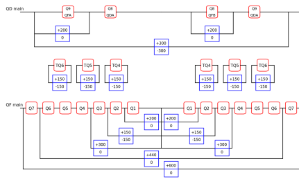
Figure 5: Schematic of the Nested Quadrupole powering scheme for RHIC interaction regions 2, 6, 8 and 12, the Q7 power supply, with 600 A, affects the current in all quadrupoles and is thus the most critical.
