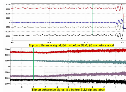
Figure 4: Illustration of BPM-MPS trips providing early detection of an ongoing failure. Top, beam oscillations caught 84 ms before an abort is issued by loss monitors. Bottom, a rising beam instability caught 8 s before loss monitors.
