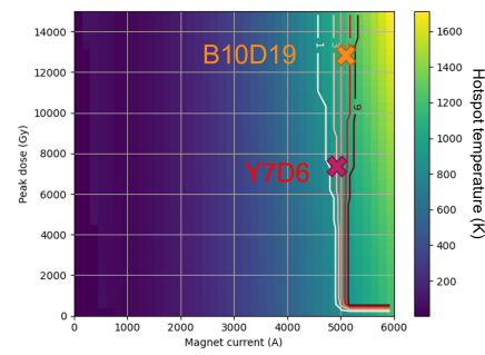
Figure 7: Parameter scan for hot-spot temperature resulting from the finite difference simulation of current crowding in bypass diodes. The contours highlight the proportion of the diode damaged during the discharge and the crosses highlight the initial conditions for two of the burnt diodes from dipole magnets.
