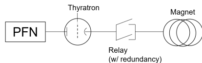
Figure 3: Schematic of the Abort Kicker triggering line with mechanical relays in series with the Pulse Forming Network and the Thyatron.
