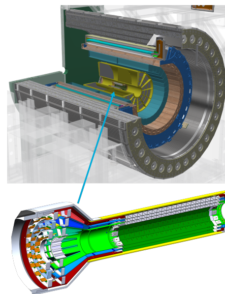
Figure 1: sPHENIX detector with MVTX vertex detector highlighted.
