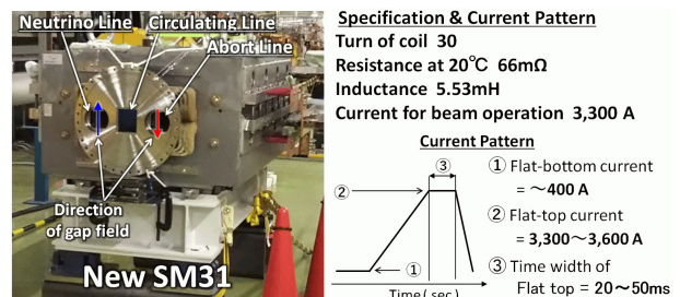
Figure 2: The photograph, the specification and the applied pattern current of the new SM31.
