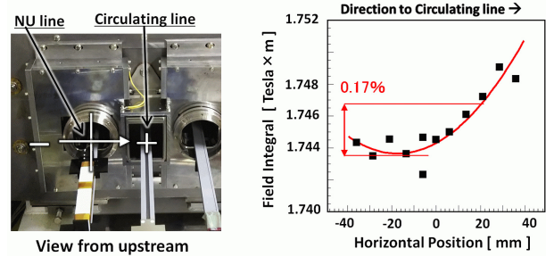
Figure 4: The view of the new SM31 from upstream (left), and the transverse distribution of the BL in the NU line, and the red curve is quadratic fit (right).
