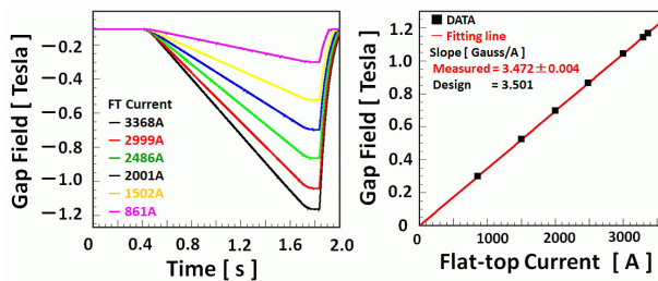
Figure 3: The waveforms of gap field in the NU line (left), and the correlation between the flat-top of the applied pattern current and the gap field (right).
