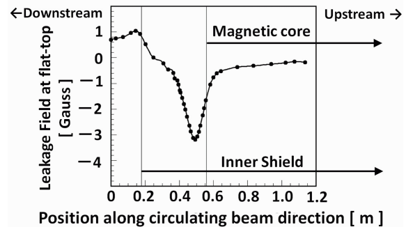
Figure 8: The additional inner shield mounted in the new SM31, viewing from downstream (upper). The longitudinal distribution of the end-fringe field along the 18-mm track with the inner shield (lower).
