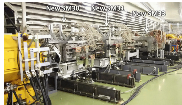
Figure 1: The high-field septa installed in MR in May 2022.
