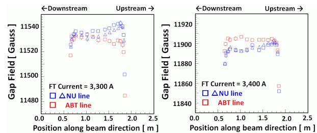
Figure 5: Comparison of longitudinal distribution of the gap field between NU and ABT line with 3,300 A (left) and 3,400 A (right).
