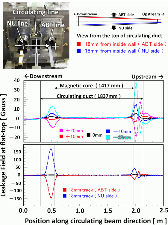
Figure 6: The longitudinal distribution of the leakage field in the circulating duct along the center track, 10-mm tracks, 25-mm tracks, and 18-mm tracks.
