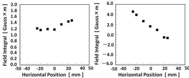
Figure 7: The horizontal position dependence of the BL: fb-BL (left) and ft-BL (right).
