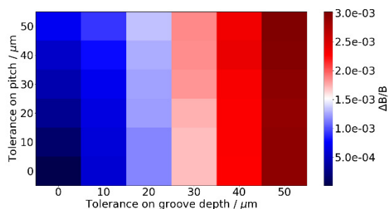
Figure 2: rms peak-to-peak field errors as function of tolerance on groove pitch and depth.
