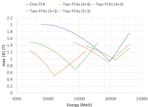
Figure 1: Maximum field on beam centroid, as a function of energy in the various FFA options.
