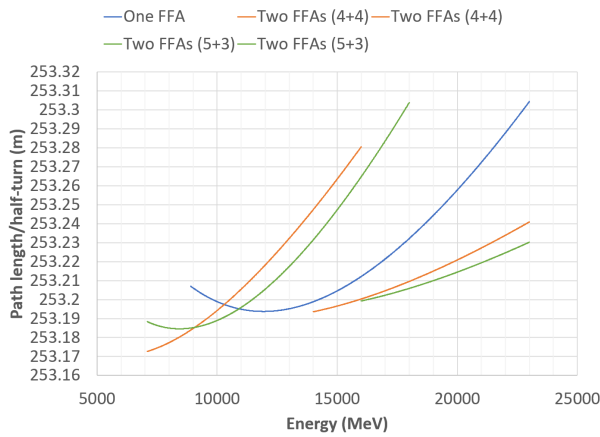
Figure 3: Path length through 180° of arc, as a function of energy in each FFA option.
