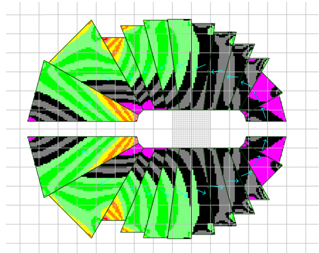
Figure 5: Sensitivity to demagnetisation in the FFA1 BD magnet, given by field antiparallel to the magnetisation direction, -\mu_0 \mathbf{H} \cdot \mathbf{M}/|\mathbf{M}| . Black is 0–0.5 T, green \leq 1 T, yellow \leq 1.5 T and red > 1.5 T. Magneta indicates parallel field.
