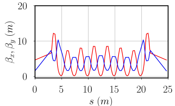
Figure 4: Betatron \beta_x (red) and \beta_y (blue) optical functions for one sector.
