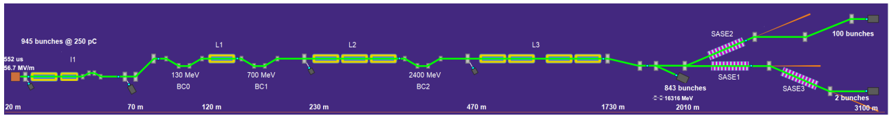
Figure 1: Schematic layout of the European X-ray Free-Electron Laser. I1: injector section; Li: the i -th linear accelerator; BC i : the i -th bunch compressor. SASE i : the i -th undulator beamlines in which SASE1 and SASE2 are hard X-ray lines while SASE3 is a soft X-ray line.
