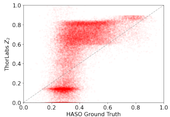
Figure 4: Raw HASO/ThorLabs correlation.
