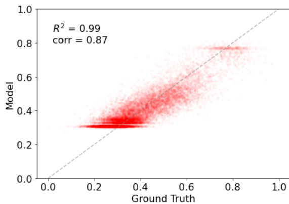
Figure 5: Feed-forward network accuracy.
