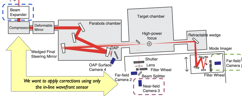
Figure 1: Diagram of HTU laser system at LBNL, highlighting the proposed correction scheme. Machine learning techniques are used to correlate a fast, non-perturbative sensor (2) with a high-quality, but perturbative wavefront sensor (1) which cannot be used for online correction. The resulting online diagnostic is used to deduce variations away from the desired focal position, which is then corrected for prior to the next shot by changes made to a transmissive lens beam expander (3).
