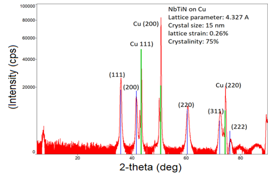
Figure 5: Grazing angle XRD of NbTiN film.
